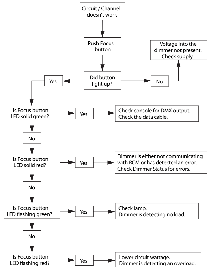
Figure 13: Troubleshooting Flow Chart
