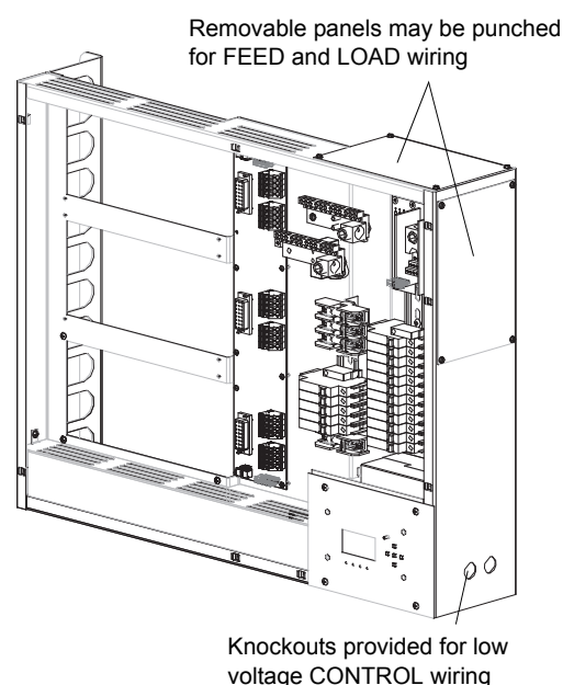
Figure 3: Wiring Inputs
