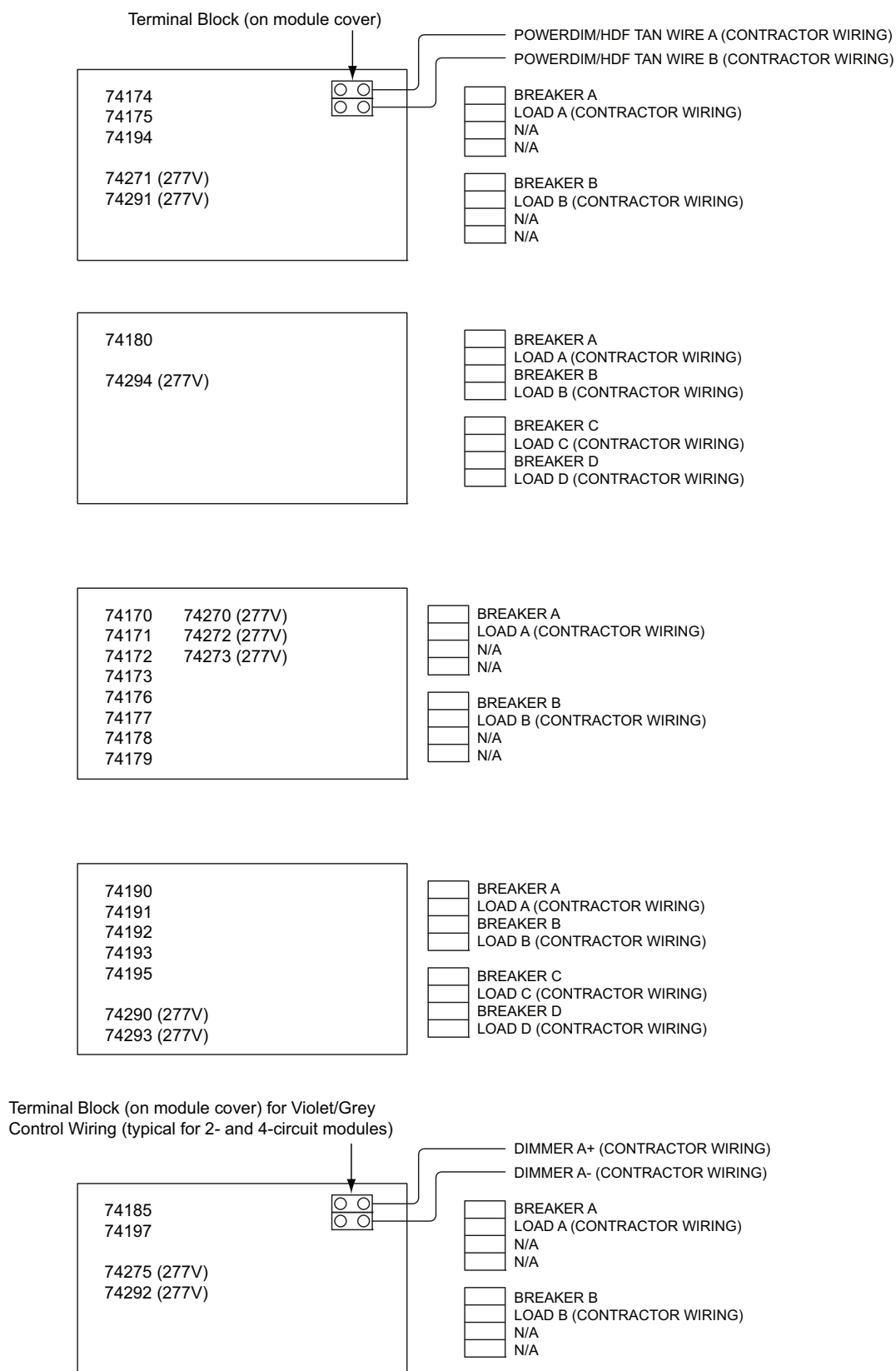
Figure 7: Module Load Wiring Diagram
