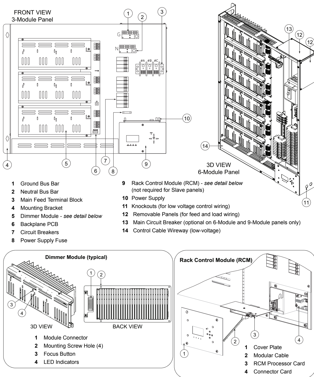
Figure 1: A21 Panel Overview
